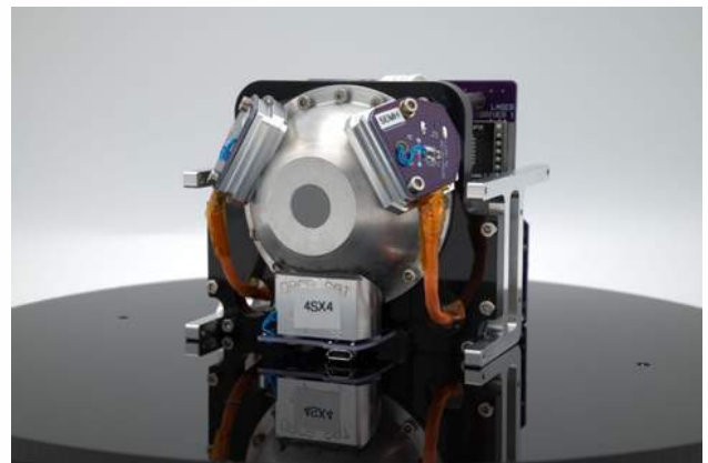
Fully assembled payload, the integrating sphere front is clearly shown with its key features.
